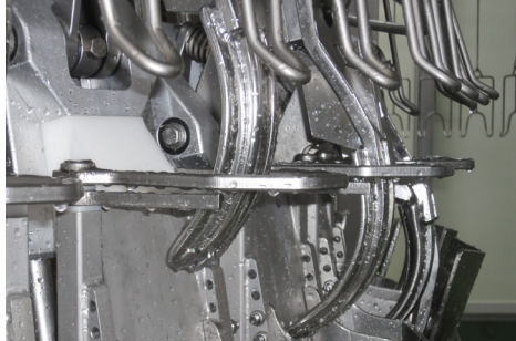
Eviscerator spoon
